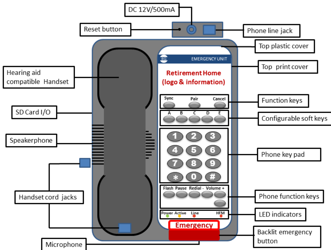
EG100 “Smart Alert Communicator” Two-Way Voice Response Station
